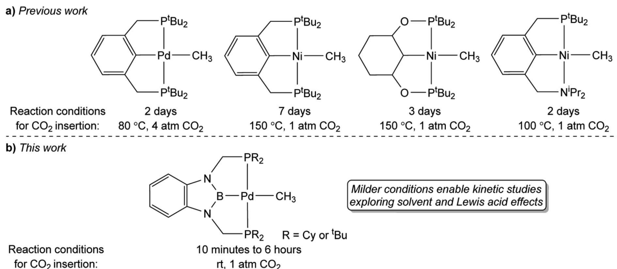
Fig. 1 (a) Previous examples of pincer-supported group 10 methyl complexes that undergo CO 2 insertion to form κ 1 -acetate complexes. (b) R PBP supported palladium complexes studied in this work, which undergo CO 2 insertion under milder conditions.
