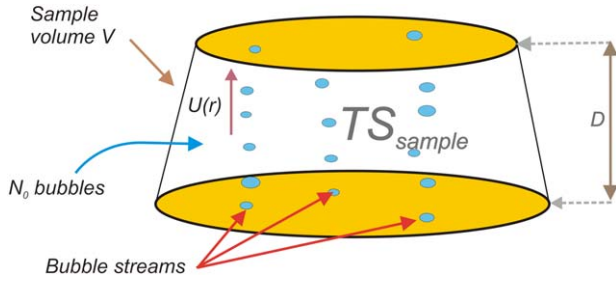
Fig. 8. Illustration of bubble streams covered by the sample volume V of the echosounder at a specific depth. Here, N_0 represents the total number of bubbles inside the sample volume V ; TS_{\text{sample}} represents the target strength of the sample volume V ; U(r) is the BRS as function of the bubble size; and D the height of the sample volume V .
