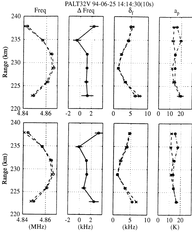
Fig. 5. The fitted parameters f_r , \Delta f_r , \delta_f and a_p as well as the error bars from the data of Fig. 4 as a function of range. The dashed-dot line is for the parameters from the upshifted line, and the dashed one is for the downshifted lines. The four upper panels show the parameters for the squared-triangle model, the four lower panels for the Gaussian model
