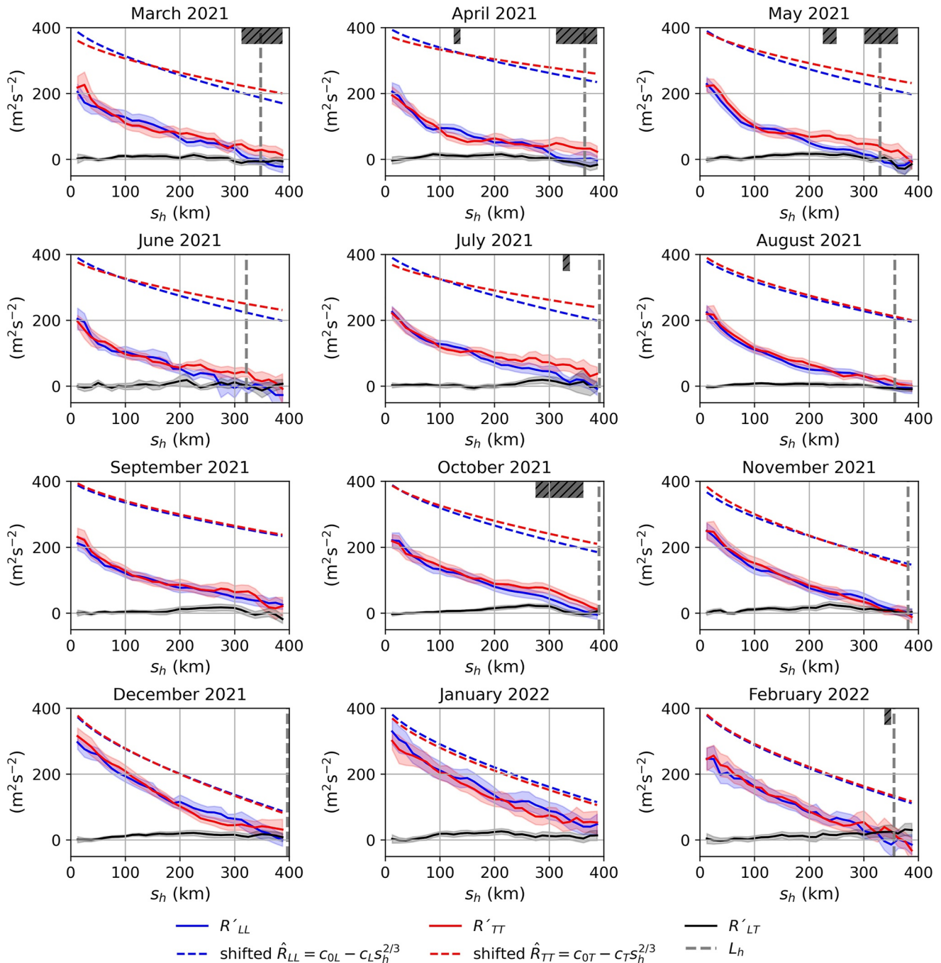
Figure 6. Monthly means of the longitudinal (blue line) and transverse (red line) correlation components of the fluctuating wind ( R'_{LL} and R'_{TT} , respectively) combining the daily curves of Figure 5. The shadowed areas mark the 90% confidence intervals. The best fits, shown with dashed lines, are shifted in the vertical direction to avoid cluttering the figure. The vertical gray lines mark the characteristic horizontal length scale of stratified turbulence L_h . Hatched boxes on top of the plots mark the s_h regions where R'_{LL} is statistically different than R'_{TT} .
