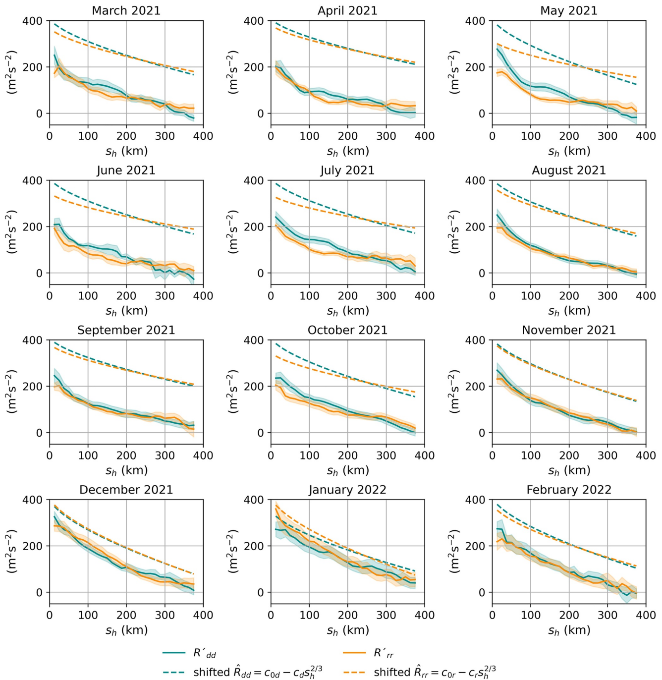
Figure 7. Monthly, divergent (cyan line) and rotational (orange line) correlation components. The shadowed areas mark the 90% confidence intervals. The best fits, shown with dashed lines, are shifted in the vertical direction to avoid cluttering the figure.
