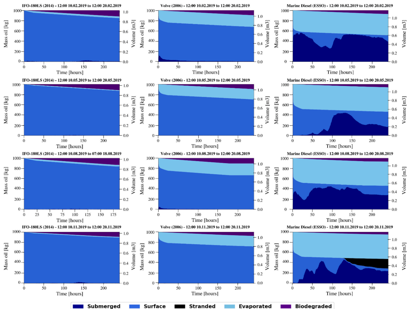
Fig. 10. Oil mass temporal balance for each type of oil in case of Svalbard: left column - heavy crude [IFO-180LS], middle column - medium crude [Volve (2006)], right column - light oil [Marine diesel (ESSO)]. Among four represented months of the year 2019 are February (top row), May and August (mid rows), and November (bottom row). The number of time-steps (240) is presented in the x-axis.
