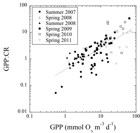
Fig. 5. The relationship between the ratio of gross primary production to community respiration (GPP/R) and gross primary production ( \text{mmol O}_2 \text{ m}^{-3} \text{ d}^{-1} ) in the different cruises. The solid line shows the fitted regression equation.
