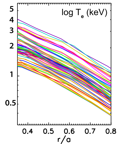
FIG. 38. Profile self-similarity is demonstrated. T_e profiles are plotted, on a semi-log scale for a random selections of shots and time including the OH, L-mode, and H-modes at a wide range in density and input power. Greenwald et al. , Fusion Sci. Tech. 51 , 266 (2007). Copyright 2007 American Nuclear Society. 185
