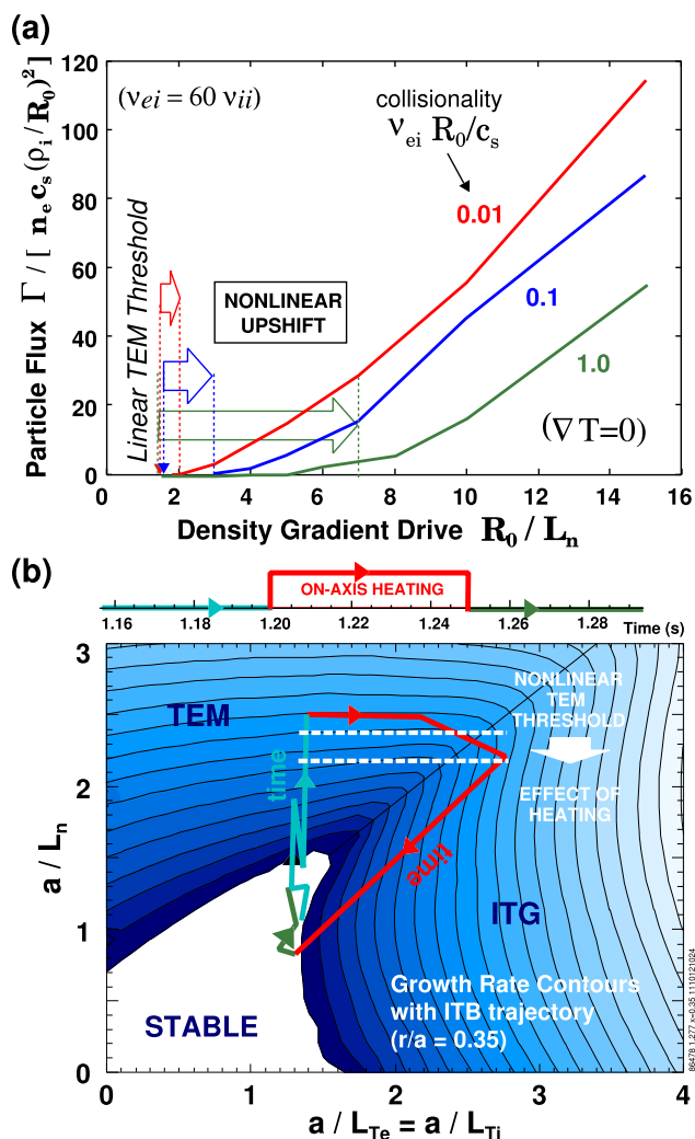
FIG. 49. A nonlinear upshift in density-gradient driven TEM was discovered in simulations of C-Mod ITB discharges. The upshift increases at higher collisionality providing a mechanism for transport control within the barrier.
