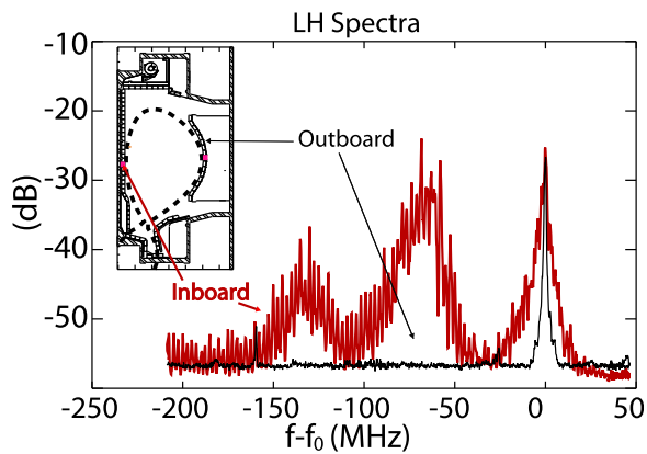
FIG. 61. Strong parametric decay is observed in measurements on the inboard (high-field) side of the machine but not on the outboard (low-field) side. This mechanism may contribute to a drop in LHCD efficiency at high density. Shiraiwa et al. , Nuclear Fusion 53 , 113028 (2013). Copyright 2013 International Atomic Energy Agency. 357
