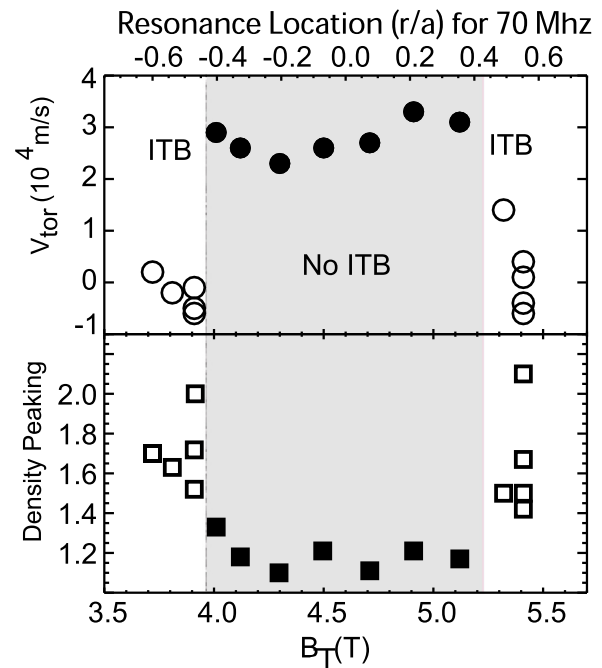
FIG. 45. ITB formation, as indicated by changes in the density profile and intrinsic rotation, depends critically on the ICRF resonance location as seen in this scan of B_T . Reprinted with permission from Fiore et al. , Fusion Sci. Tech. 51 , 303 (2007). Copyright 2007 American Nuclear Society. 248
