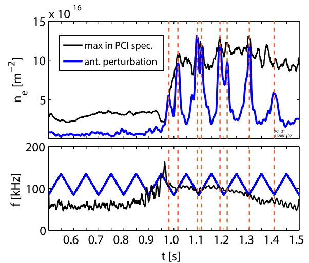
FIG. 36. The magnetic perturbation applied by the shoe-lace antenna drives a strong plasma density response when the drive frequency is at or near resonance with the naturally occurring QCM. Reproduced with permission from Phys. Plasmas 21 , 056111 (2014). Copyright 2014 AIP Publishing LLC. 113
