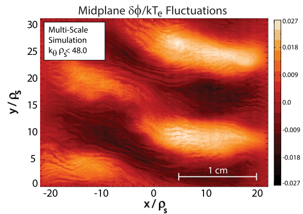
FIG. 48. Multi-scale gyrokinetic simulations, which include both electron and ion-scale dynamics show that fine scale ETG streamers can coexist with larger ITG structures and produce electron heat flux consistent with experiments.
