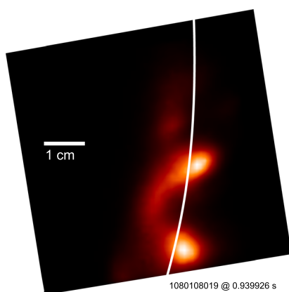
FIG. 16. The far-SOL plasma is composed of large amplitude structures (often called “blobs” or “filaments”) that originate in the near-SOL and propagate poloidally and radially. This image is produced by the gas-puff imaging (GPI) diagnostic.
