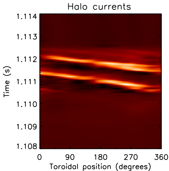
FIG. 64. C-Mod demonstrated that the toroidal structure of halo currents rotated rapidly, likely in response to the motion of the disrupting plasma. In this plot, the magnitude of halo currents in space and time is indicated by image brightness.
