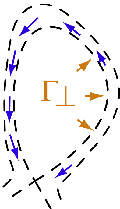
FIG. 20. Schematic showing how asymmetric transport drives sonic flows in the SOL.
