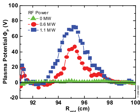
FIG. 55. Significant RF sheath potentials are measured with an amplitude proportional to input power. The acceleration of ions through this sheath and onto the first wall is believed to contribute to the increased impurity content of ICRF heating plasmas.
