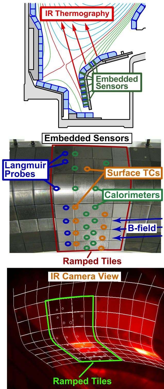
FIG. 10. Divertor heat flux diagnostics. Reproduced with permission from Phys. Plasmas 18 , 056104 (2011). Copyright 2011 AIP Publishing LLC. 72
