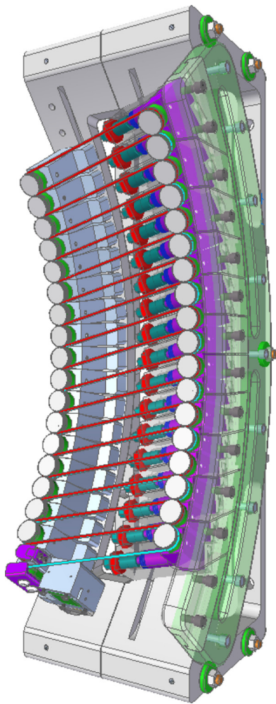
FIG. 35. A 3D rendering of the “shoelace” antenna, which can drive short wavelength magnetic perturbations in the plasma edge.
