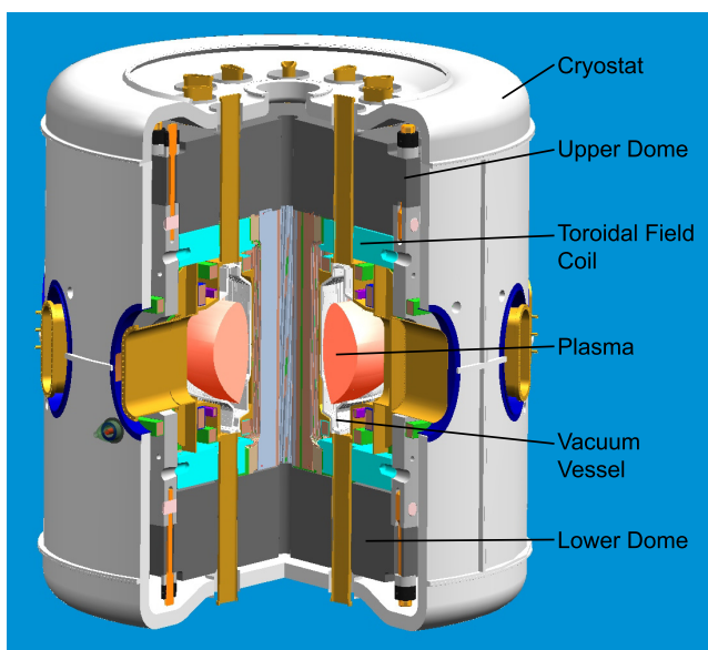
FIG. 2. A schematic of the C-Mod tokamak showing the major components.
