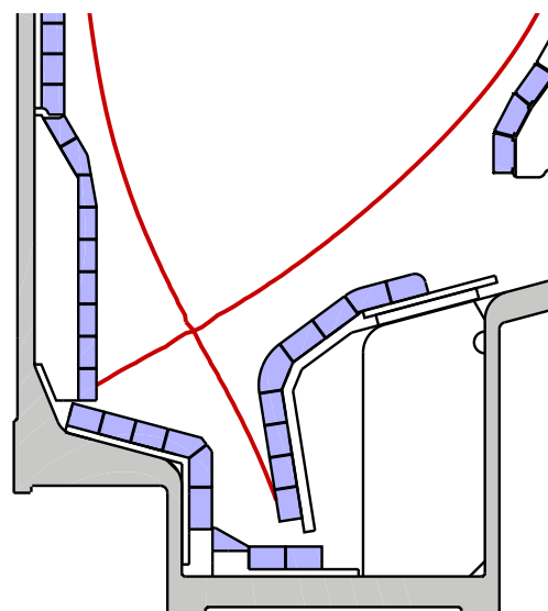
FIG. 4. The C-Mod vertical target divertor features a small incident angle between the magnetic field and the wall, a long divertor leg and natural baffling of neutrals. The separatrix for a typical MHD equilibrium is plotted in red.
