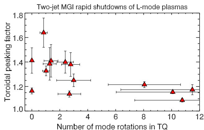
FIG. 70. C-Mod data shows that time-averaged radiation symmetry can be achieved in a disruption if the MHD modes rotate many times during the quench. For discharges where the rotation is slower compared to the disruption speed, the asymmetry becomes prominent. The prediction of radiation asymmetry in ITER mitigated disruption thus becomes dependent on predictions of plasma rotation during the disruption.
