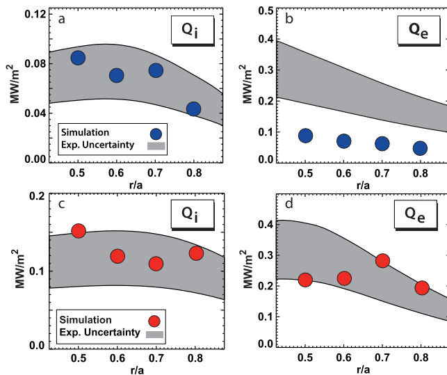
FIG. 47. Experimental ion and electron heat fluxes are shown for low-power (blue— (a), (b)) and high-power (red—(c), (d)) L-modes. The ion transport matches ion-scale gyrokinetic simulations at all radii, not showing the “shortfall” reported on DIII-D. At high powers, TEM instabilities in the simulation are excited and can explain electron heat transport. A discrepancy remains in the low-power case. Reproduced with permission from Phys. Plasmas 20 , 032510 (2013). Copyright 2013 AIP Publishing LLC. 269
