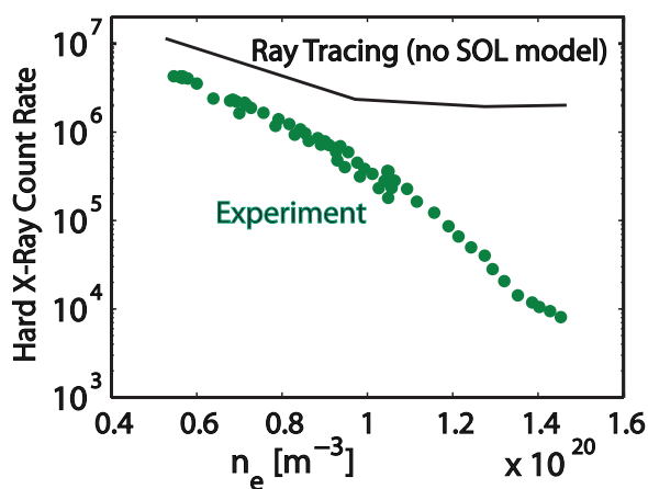
FIG. 59. At high densities, but below wave accessibility limits, driven current—indicated here by the decrease in hard x-rays—drops well below the expectations of a simple ray tracing model. Reproduced with permission from Phys. Plasmas 19 , 062505 (2012). Copyright 2012 AIP Publishing LLC. 359
