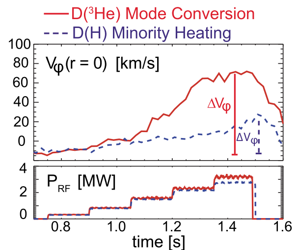
FIG. 54. ICRF flow drive is demonstrated in this comparison of minority heating (blue) with only intrinsic rotation (which is proportional to plasma energy) and mode-conversion heating (red). With equal power in each regime, significantly higher flow is produced in the mode conversion case. Reproduced with permission from Phys. Plasmas 16 , 056102 (2009). Copyright 2009 AIP Publishing LLC. 316
