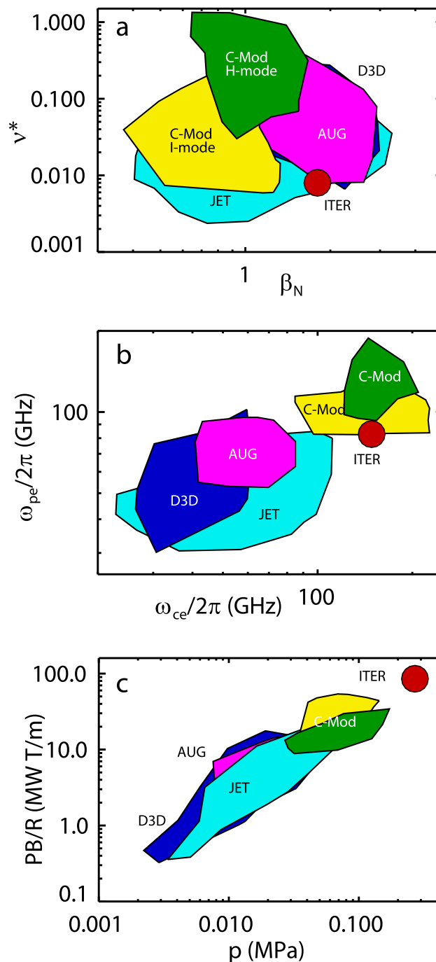
FIG. 1. C-Mod parameters are compared to other tokamaks and those projected for ITER as relevant to physics for (a) core MHD, (b) RF heating and current drive, and (c) boundary plasma physics where PB/R is a proxy for the divertor heat load and the core pressure a proxy for the divertor pressure. Data are mainly from the ITPA H-mode data base and includes C-Mod I-modes for comparison.
