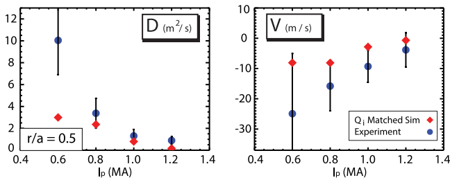
FIG. 51. Impurity transport coefficients, D_z , V_z , from an I_p are compared to gyrokinetic simulations which match the values and trends found in the experiments. Reproduced with permission from Phys. Plasmas 19 , 056110 (2012). Copyright 2012 AIP Publishing LLC. 268
