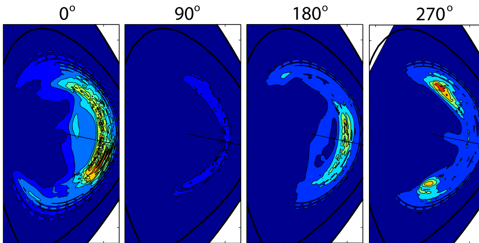
FIG. 69. Radiation patterns from 4 different toroidal locations from NIMRAD modeling of a mitigated disruption are shown. This strong 3D spatial structure is generally consistent with measurements, but the model cannot predict rotation from first principles.
