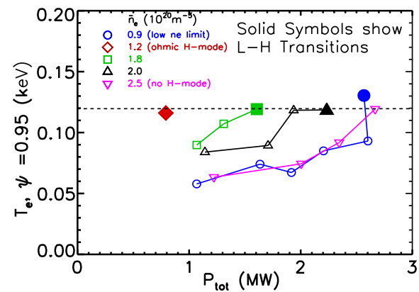
FIG. 22. The L-H transition was found to have a sharp threshold at a fixed temperature independent of density. 137 Reprinted with permission from Hubbard et al. , in Proceedings of the 16th International Atomic Energy Agency Conference on Fusion Energy (IAEA, Montreal, 1996), Vol. 1, p. 875. Copyright 1996 IAEA.
