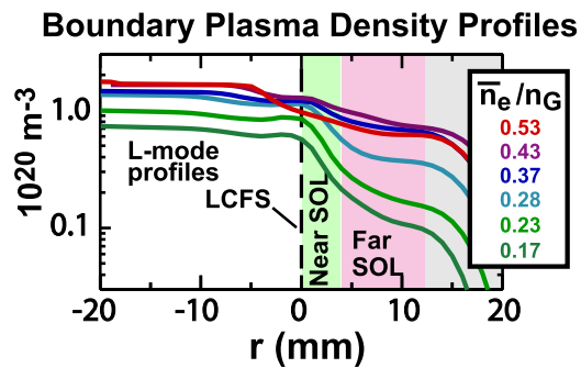
FIG. 9. Typical SOL density profile as a function of global normalized density. Reproduced with permission from Phys. Plasmas 15 , 056106 (2008). Copyright 2008 AIP Publishing LLC. 91
