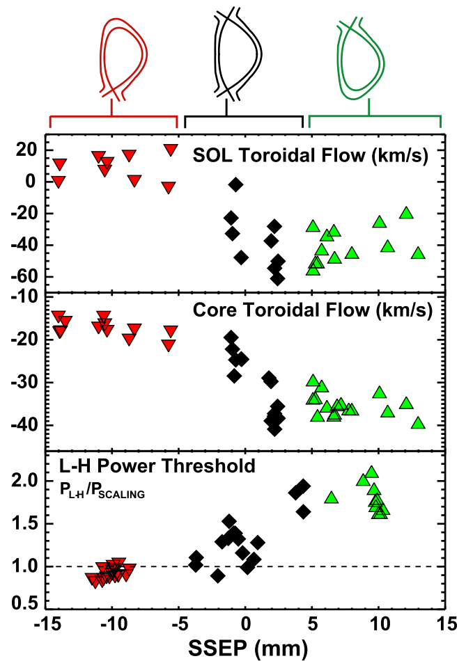
FIG. 24. The L-H power threshold is well-correlated with the topology dependent flows seen in the plasma edge and core. The independent axis, SSEP is the distance between the primary and secondary separatrices, mapped to the midplane. Reproduced with permission from Phys. Plasmas 12 , 056111 (2005). Copyright 2005 AIP Publishing LLC. 113
