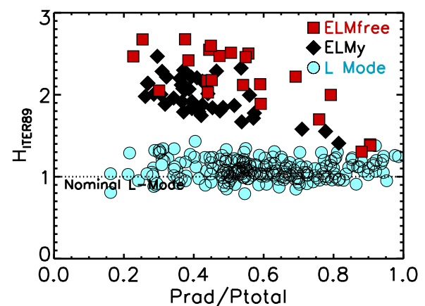
FIG. 39. Normalized energy confinement for the L-mode can be maintained, even at very low levels of conducted power. In contrast, the H-mode confinement deteriorates at a high radiated power because of the decrease in pedestal temperature. Reprinted with permission from Greenwald et al. , Nuclear Fusion 37 , 793 (1997). Copyright 1997 IOP. 17
