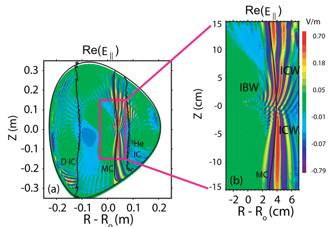
FIG. 52. TORIC simulations of ICRF propagation show the incoming fast wave, the anticipated, mode-converted, forward-propagating IBW and the re-discovered, backward propagating ICW. Lin et al. , Plasma Physics and Controlled Fusion 47 , 1207 (2005). Copyright 2005 International Atomic Energy Agency. 309
