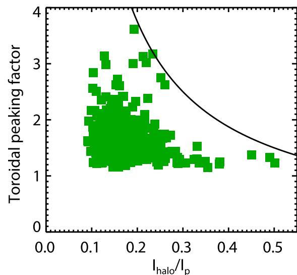
FIG. 63. Toroidal peaking of halo currents is lower for discharges with the highest conversion of plasma current to halo current, but the stresses on machine components can be dangerous over much of this range.
