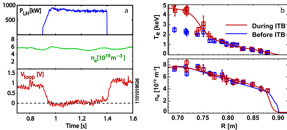
FIG. 58. (a) Efficient LHCD can produce fully non-inductive discharges at densities above 0.5 \times 10^{20} . Reproduced with permission from Phys. Plasmas 19 , 062505 (2012). Copyright 2012 AIP Publishing LLC. 359 (b) Off axis-current drive can modify the magnetic shear and allow an electron ITB to form. Shiraiwa et al. , Nuclear Fusion 53 , 113028 (2013). Copyright 2013 International Atomic Energy Agency. 357
