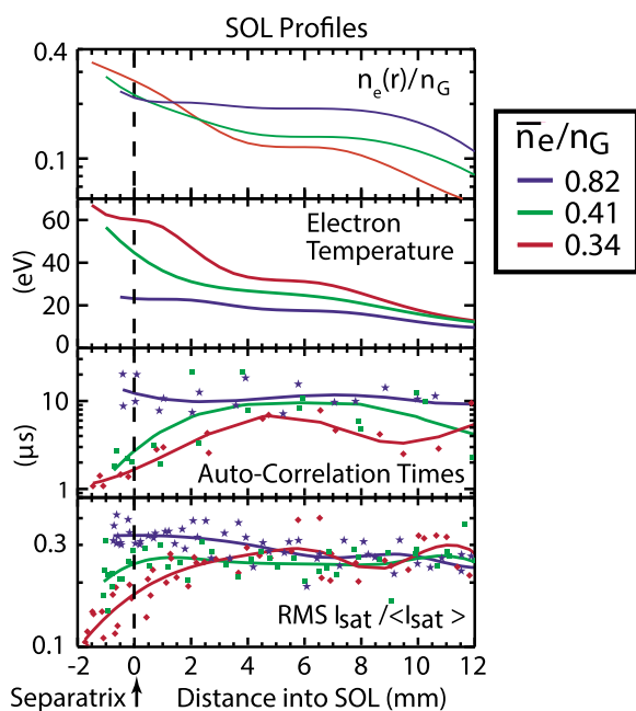
FIG. 18. Probe measurements show the increase in turbulence amplitude and intermittency that occurs as the normalized density n_e/n_G is raised. Reproduced with permission from Phys. Plasmas 8 , 2107 (2001). Copyright 2001 AIP Publishing LLC. 87
