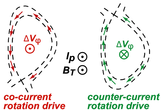
FIG. 23. The direction of SOL flows driven by poloidally asymmetric radial transport depends only on the direction of the \nabla B drift relative to the direction to the x-point. For all combinations of toroidal field, plasma current or X-point direction. Reprinted with permission from LaBombard et al. , Nuclear Fusion 44 , 1047 (2004). Copyright 2004 IOP. 112
