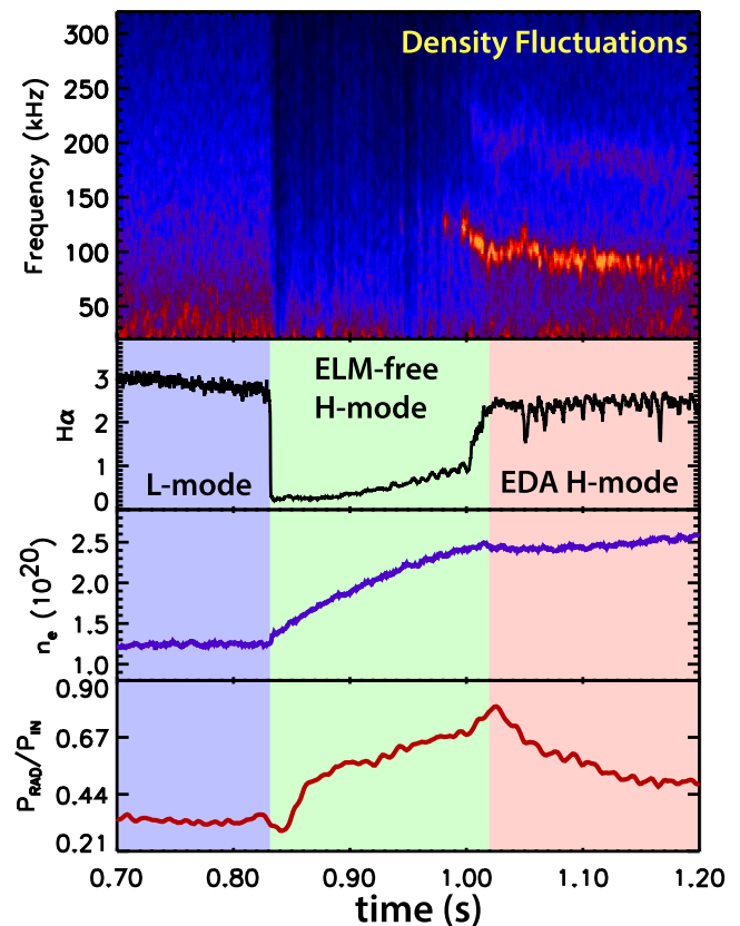
FIG. 26. A sudden transition from the ELM-free to the EDA H-mode is accompanied by a change in impurity confinement and the appearance of the QCM. Greenwald et al. , Fusion Sci. Tech. 51 , 266 (2007). Copyright 2007 American Nuclear Society. 185
