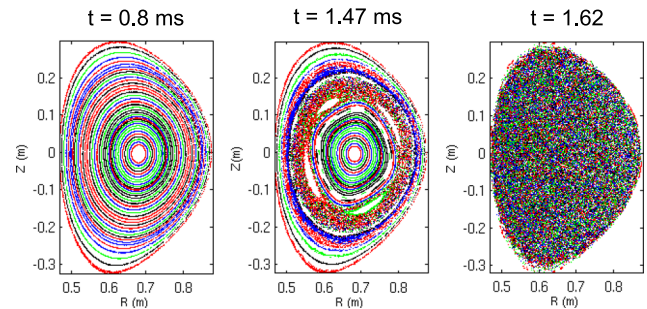
FIG. 67. Nonlinear MHD modeling with the combined NIMRAD code shows the evolution of the field structure throughout a mitigated disruption. The first panel shows the unperturbed flux surfaces that exist before edge cooling begins to destabilize the plasma. The second panel shows large magnetic islands and stochastic regions driven by the growth in MHD modes as the current channel shrinks. The last panel shows complete stochasticization of the field structure just 150 \mu s later. Time is measured from the triggering of the MGI system. Reproduced with permission from Phys. Plasmas 15 , 056109 (2008). Copyright 2008 AIP Publishing LLC. 178
