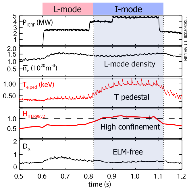
FIG. 28. The transition from the L to I-mode is shown, demonstrating the increase in energy confinement without a change in particle transport or the appearance of ELMs. 179 Reprinted with permission from Hubbard et al. , in Proceedings of the 24th IAEA Fusion Energy Conference (IAEA, San Diego, 2012), see http://www-naweb.iaea.org/naweb/physics/FEC/FEC2012/papers/171_EX13.pdf . Copyright 2012 IAEA.
