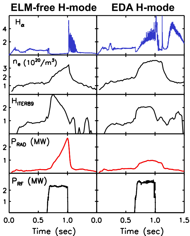
FIG. 27. A comparison of waveforms between the ELM-free and the EDA H-modes shows the essential stationary character of the EDA and the drop in particle and impurity transport. Greenwald et al. , Fusion Sci. Tech. 51 , 266 (2007). Copyright 2007 American Nuclear Society. 185
