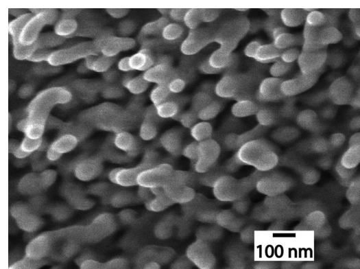
FIG. 6. A micrograph of tungsten nanostructures produced by 13 s of helium discharge time on a target operating at about 2000 K. The morphology and growth rate are essentially identical to what is produced in a linear plasma device under similar conditions. Reprinted with permission from Wright et al. , Nuclear Fusion 52 , 042003 (2012). Copyright 2012 IOP. 51
