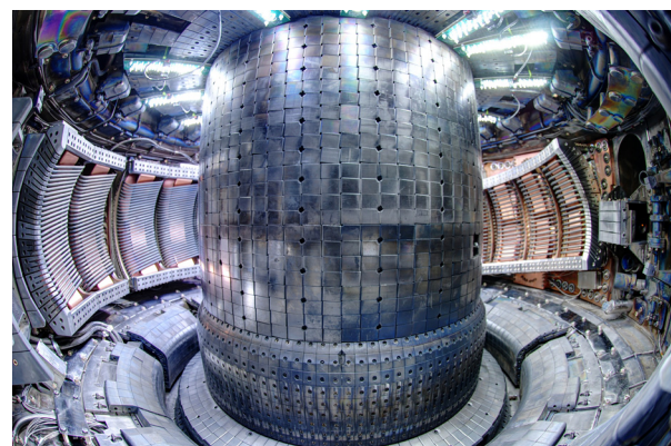
FIG. 3. Photo taken inside C-Mod, showing internal components including the divertor and inner wall limiter tiles as well as ICRF antennas and numerous diagnostics.
