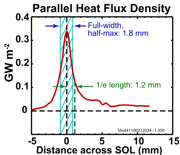
FIG. 11. The heat flux profile measured with the infra-red camera and calibrated against probes and thermocouples. These profiles show the narrowest width and highest power flux measured on any magnetic confinement experiment. Reproduced with permission from Phys. Plasmas 18 , 056104 (2011). Copyright 2011 AIP Publishing LLC. 72
