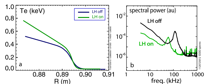
FIG. 34. (a) The increase in the temperature pedestal after the application of a small increment in RF power in the lower-hybrid range of frequencies applied to plasmas strongly heated by ICRF. (b) The increase in temperature is accompanied by a drop of almost an order of magnitude in edge fluctuations.
