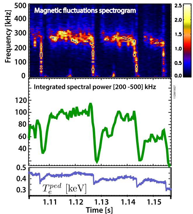
FIG. 33. Magnetic fluctuations are shown to grow rapidly as the plasma temperature recovers between the ELMs. These fluctuations may be evidence for kinetic ballooning, a key element in the EPED model for pedestal structure. Hughes et al. , Nuclear Fusion 53 , 8, 043016 (2013). Copyright 2013 International Atomic Energy Agency. 154
