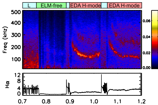
FIG. 31. The density fluctuation spectra are shown for a discharge with three H-mode periods. The first is ELM-free followed by two EDA intervals with the presence of a strong QCM. Greenwald et al. , Fusion Sci. Tech. 51 , 266 (2007). Copyright 2007 American Nuclear Society. 185
