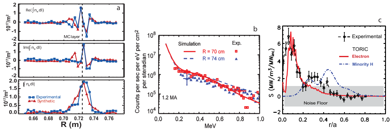
FIG. 53. (a) Mode-converted RF waves measured with phase-contrast imaging are compared to full-wave simulations. Lin et al. , Plasma Physics and Controlled Fusion 47 , 1207 (2005). Copyright 2005 International Atomic Energy Agency. 309 (b) The energy spectra of non-thermal ions are compared to AORSA simulations of minority heating. These simulations show agreement in the equilibrium distribution function as well as its dependence on plasma current and input power. Reproduced with permission from in Proceedings of the 19th Topical Conference on Radio Frequency Power in Plasmas (2011), Vol. 1406. Copyright 2011 AIP Publishing LLC. 341 (c) Experimental measurements of local heat deposition are compared to TORIC simulations of mode conversion heating. Lin et al. , Plasma Physics and Controlled Fusion 45 , 1013 (2003). Copyright 2003 International Atomic Energy Agency. 299
