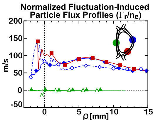
FIG. 19. Normalized turbulent flux profiles from the low- and high-field side of the discharge are compared. There is essentially no turbulent transport on the high-field side of the tokamak, consistent with an important curvature drive for the underlying instabilities. Smick et al. , Nuclear Fusion 53 , 023001 (2013). Copyright 2013 International Atomic Energy Agency. 114
