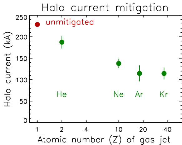
FIG. 65. The magnitude of halo currents could be reduced by injection of large quantities of noble gases. For purer gases, the effectiveness generally increased with atomic number, but the best results were obtained with a mix of helium (90%) and argon (10%). Reprinted with permission from Granetz et al. , Nuclear Fusion 46 , 1001 (2006). Copyright 2006 IOP. 379
