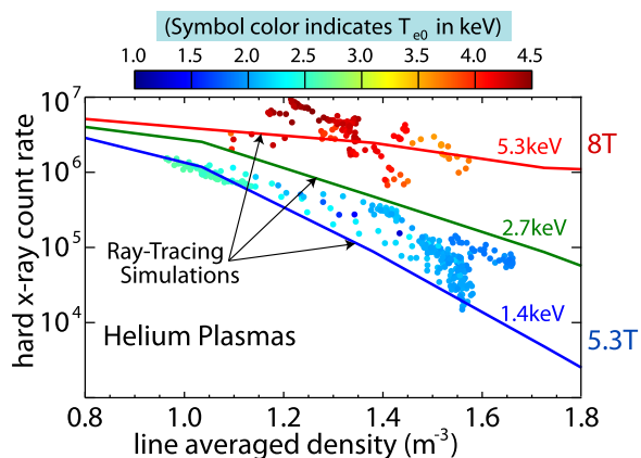
FIG. 62. Improved performance at high densities with higher temperatures. Shiraiwa et al. , Nuclear Fusion 53 , 113028 (2013). Copyright 2013 International Atomic Energy Agency. 357
