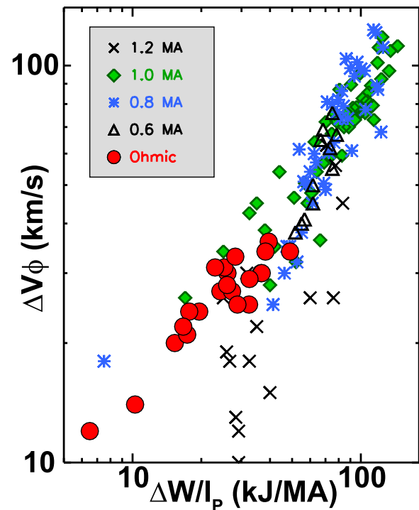
FIG. 40. Intrinsic rotation scales with stored energy divided by the plasma current and is independent of the heating method. Reprinted with permission from Rice et al. , Nuclear Fusion 41 , 277 (2001). Copyright 2001 IOP. 251
