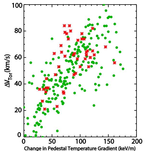
FIG. 41. Intrinsic toroidal rotation is proportional to the pedestal temperature gradient for both H-modes (green) and I-modes (red), consistent with the model that this rotation is driven by residual stress. Rice et al. , Phys. Rev. Lett. 106 , 265001 (2011). Copyright 2011 American Physical Society. 213
