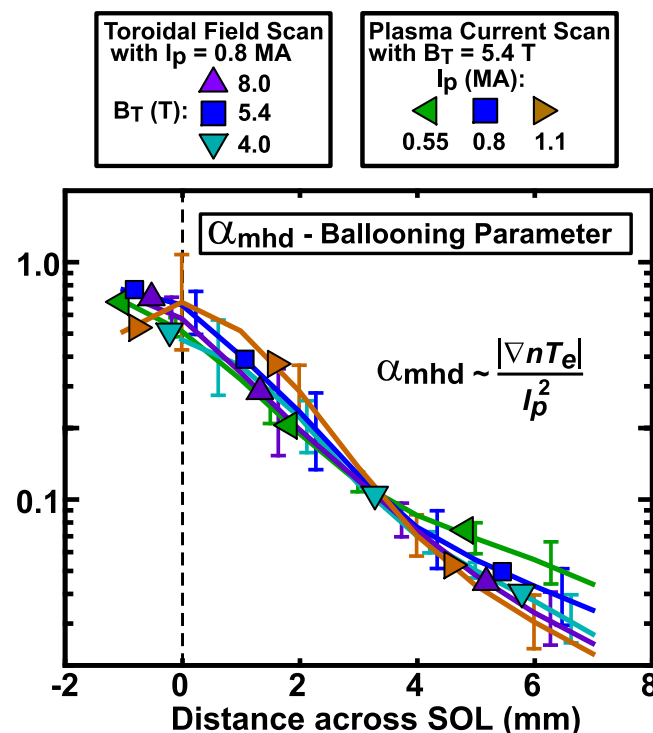
FIG. 14. Plasma profiles in the SOL overlay if they are parameterized by the \alpha_{MHD} parameter (essentially the gradient in \beta_P ) supporting the hypothesis that the profiles are set by cross field transport at marginal stability. Reproduced with permission from Phys. Plasmas 18 , 056104 (2011). Copyright 2011 AIP Publishing LLC. 72
