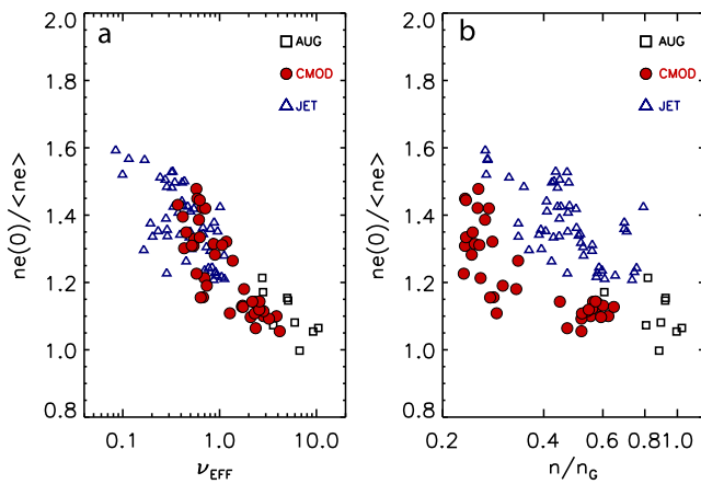
FIG. 43. Density peaking ratios in C-Mod is overlaid on data from AUG and JET showing that the appropriate scaling is collisionality (a) rather than n/n_G (b) thus implying a moderate level of peaking for ITER baseline discharges. Reprinted with permission from Greenwald et al. , Nuclear Fusion 47 , L26 (2007). Copyright 2007 IOP. 182
