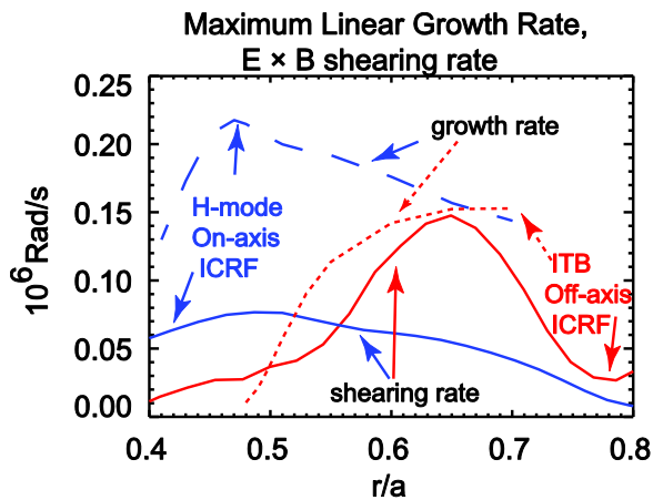
FIG. 46. The E \times B shearing rate from intrinsic rotation can reach the ITG growth rate for discharges with off-axis ICRF that transition to an ITB. In similar H-mode discharges, with on-axis heating, the E \times B rate is far below the growth rate. Reproduced with permission from Phys. Plasmas 19 , 056113 (2012). Copyright 2012 AIP Publishing LLC. 217
