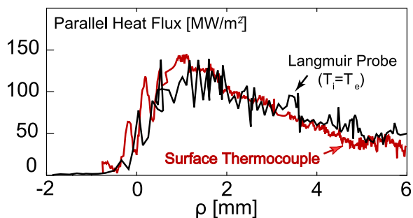
FIG. 12. Heat flux profiles calculated based on plasma measurements compare well to the values taken directly from surface diagnostics. Reproduced with permission from Rev. Sci. Instrum. 83 , 033501 (2012). Copyright 2012 AIP Publishing LLC. 74
