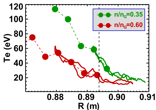
FIG. 17. Edge temperature profiles show the progressive edge cooling as the normalized density is increased toward n_G .
