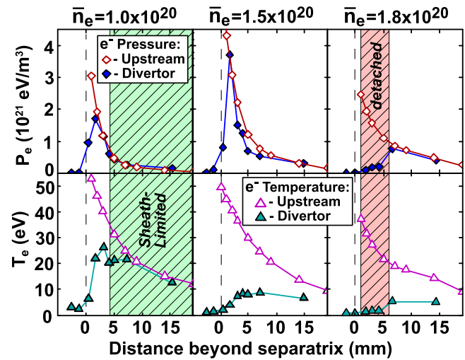
FIG. 8. Three divertor regimes that are produced at increasing density, are identified in this plot of pressure and temperature profiles in the SOL. Reproduced with permission from Phys. Plasmas 2 , 2242 (1995). Copyright 1995 AIP Publishing LLC. 58
