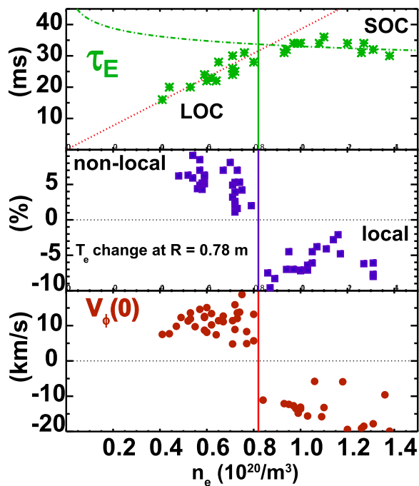
FIG. 42. Reversal of intrinsic rotation occurs dramatically at a q -dependent, critical density. The transition from LOC-SOC confinement and from non-local to local transient transport occur at the same density. Reprinted with permission from Rice et al. , Nuclear Fusion 53 , 033004 (2013). Copyright 2013 IOP. 225
