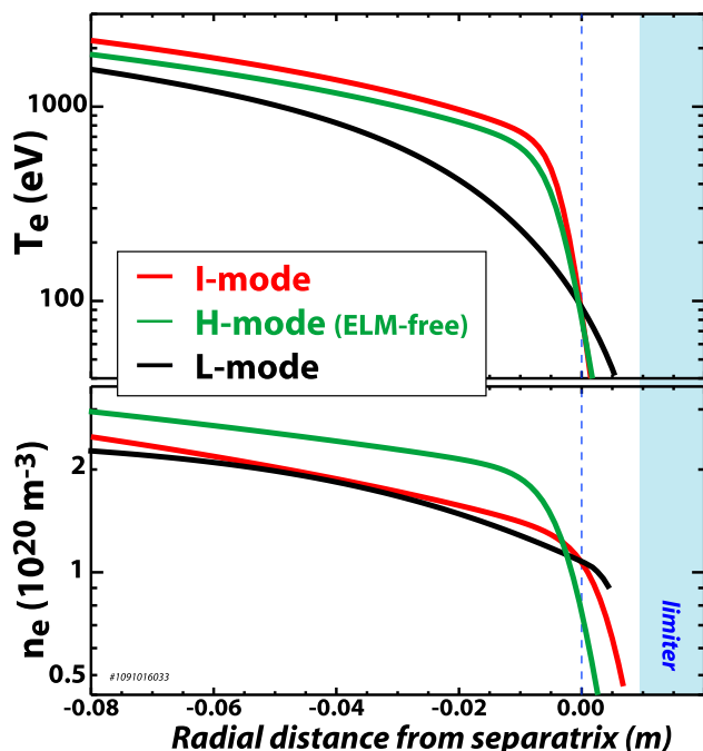
FIG. 29. The profiles of electron temperature and density are compared for the L-mode, H-mode, and I-mode.
