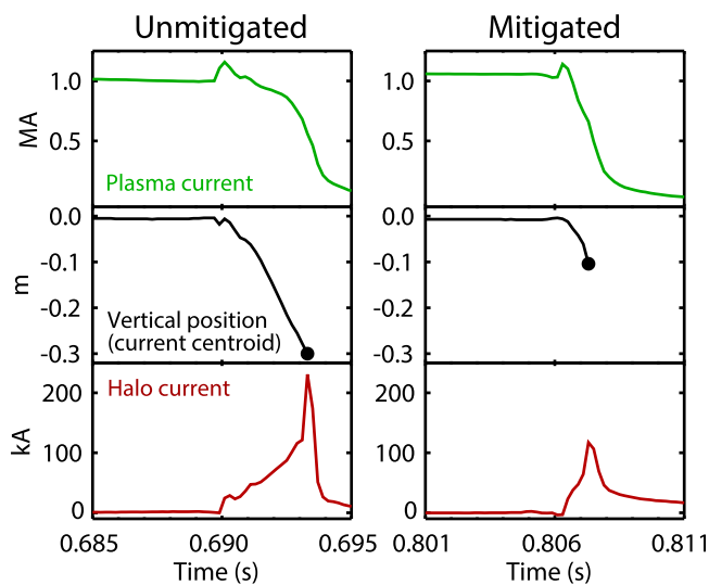
FIG. 66. This data demonstrate the mechanism of halo current mitigation. The massive gas injection leads to a faster current quench and thus to less vertical motion before the quench is complete. Reprinted with permission from Granetz et al. , Nuclear Fusion 46 , 1001 (2006). Copyright 2006 IOP. 379
