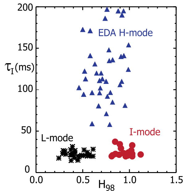
FIG. 30. The confinement times of calcium impurities, injected via the laser blow-off technique, are plotted vs normalized energy confinement and confirm the L-mode-like particle transport for the I-mode plasmas.
