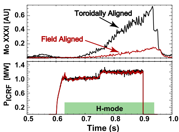
FIG. 57. The molybdenum source rate during ICRF heating drops by almost an order of magnitude in FA design. Reproduced with permission from Phys. Plasmas 20 , 056117 (2013). Copyright 2013 AIP Publishing LLC. 295
