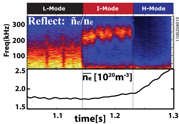
FIG. 32. Density fluctuations are shown a discharge transitions from the L- to I- to H-mode. The I-mode is typically accompanied by the appearance of a WCM at frequencies above 200 kHz and the reduction in lower frequency fluctuations. Reproduced with permission from Phys. Plasmas 18 , 056115 (2011). Copyright 2011 AIP Publishing LLC. 152
