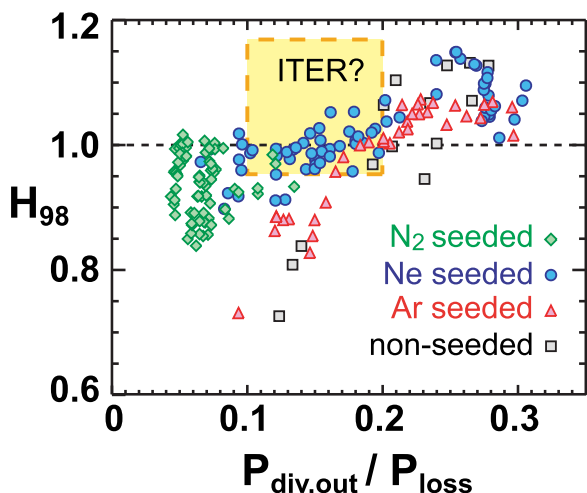
FIG. 13. Normalized H-mode confinement, H_{98} is plotted vs P_{div}/P_{loss} , the power conducted to the divertor normalized to the net input power. By puffing small amounts of impurities, radiation losses can be increased without degrading confinement—meeting ITER operational requirements. Reprinted with permission from Hughes et al. , Nuclear Fusion 51 , 083007 (2011). Copyright 2011 IOP. 83
