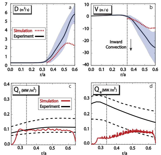
FIG. 44. Profiles of impurity transport coefficients, D_z (a) V_z (b), are obtained from impurity injection experiments. These are compared to gyrokinetic simulations, which can simultaneously match the ion energy (c) and impurity particle transport within experimental uncertainties. Electron energy transport is under-predicted in these simulations (d). Reproduced with permission from Phys. Plasmas 19 , 056110 (2012). Copyright 2012 AIP Publishing LLC. 268
