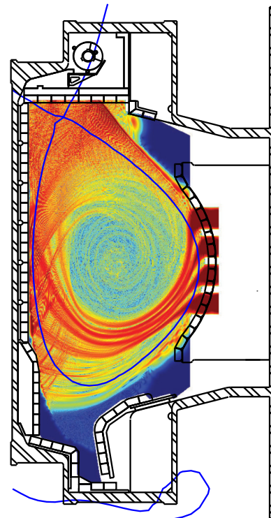
FIG. 60. A full-wave LH simulation at high density, showing waves propagating in the edge plasma.
