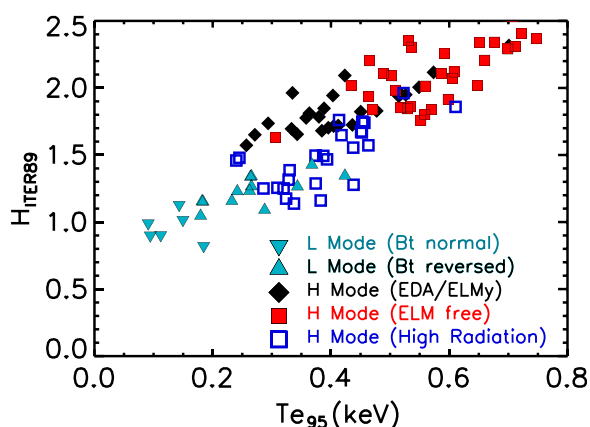
FIG. 37. The energy confinement time, normalized to the ITER89 L-mode scaling law, is plotted vs the pedestal temperature, unifying data over a wide range of parameters and confinement regimes. Reprinted with permission from Greenwald et al. , Nuclear Fusion 37 , 793 (1997). Copyright 1997 IOP. 17
