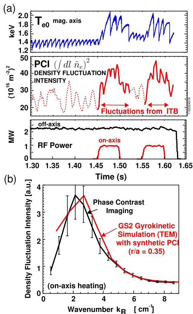
FIG. 50. Modulated on-axis heating in ITB discharges allows measured fluctuations to be localized within the barrier and supports the theory of barrier control via density gradient driven TEMs.
