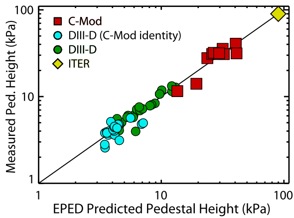
FIG. 25. The measured profile structure is consistent with the EPED model, extending the world database to within a factor of three of what is expected on ITER. Hughes et al. , Nuclear Fusion 53 , 8, 043016 (2013). Copyright 2013 International Atomic Energy Agency. 154
