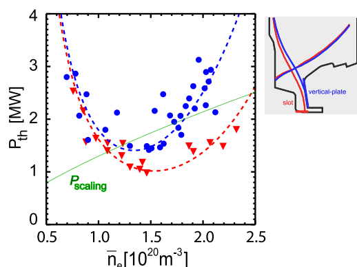
FIG. 21. The L-H power threshold vs plasma density has a distinct minimum and rises faster than linearly on either side. A strong dependence of the threshold on divertor topology is found on the high density side. Greenwald et al. , Nuclear Fusion 53 , 14, 104004 (2013). Copyright 2013 International Atomic Energy Agency. 197
