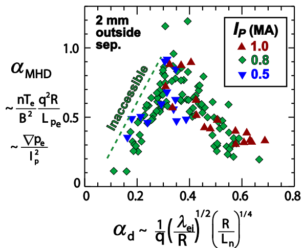
FIG. 15. The normalized pressure gradient ( \alpha_{\text{MHD}} ) in the near-SOL depends on strongly on collisionality. 88 Reprinted with permission from LaBombard et al. , Nuclear Fusion 45 , 1658 (2005). Copyright 2005 IOP. \alpha_d is the inverse normalized collisionality as defined in Ref. 90.
