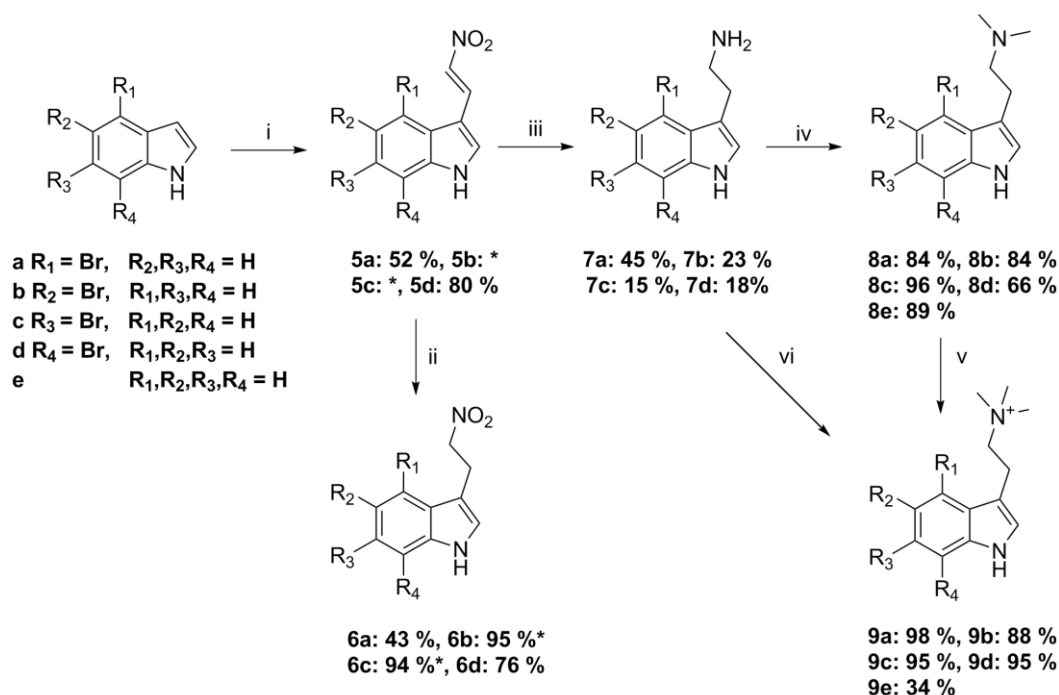
Scheme 1. Reagents, solvents, conditions and isolated yield: (i) N,N -dimethylamino nitroethylene, TFA, (ii) H 3 BO 3 , NaBH 4 , THF, isopropanol (iii) LiAlH 4 , THF, (iv) acetic acid, NaBH 3 CN, formaldehyde (v) MeI, CHCl 3 (vi) MeI, isopropanol. *Yield over two steps reported.
